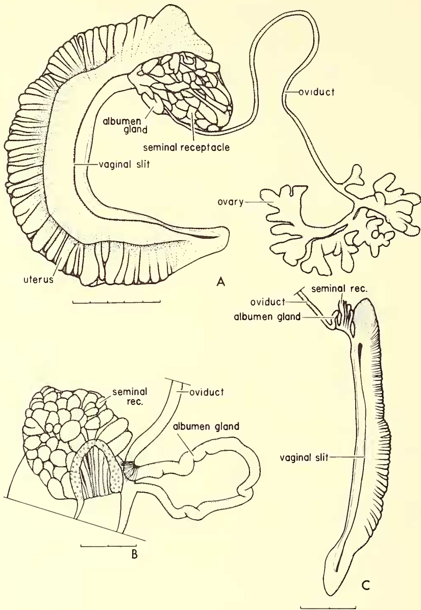
TEXT-FIG. 2. Female reproductive systems of two species of Aperostominae. A. Farcimen croteum (Gmelin); 2.5 mi. s.w. Yabucoa, Puerto Rico. B. Farcimen croteum (Gmelin); enlarged view of seminal receptacle with the receptacle chamber partially opened. The albumen gland has been partially freed from the side of the receptacle. C. Aperostoma mexicana salleana (Martens); 4.3 mi. e. Cordoba, Veracruz. Scale for A equals 5 mm; scales for B and C equal 2 mm.
